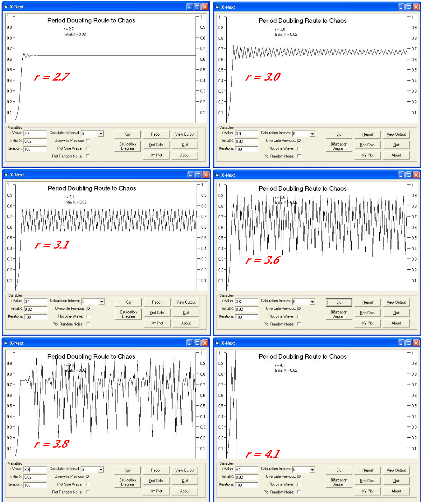
Figure 1 - Series of 100 generation time series diagrams generated by the logistic system at increasing values of 'r'. Note how the behavior becomes more energetic and complex as the 'r' values increase until the system self-destructs and goes extinct at a 'r' value between 4.0 and 4.1.
