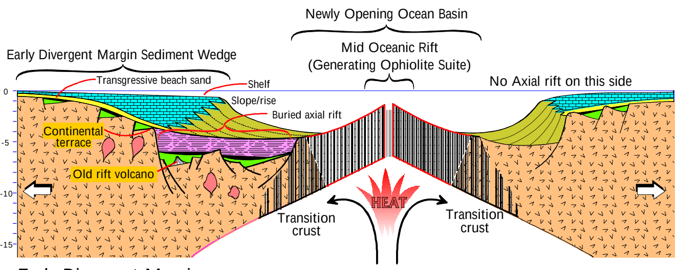
Early Divergent Margin
