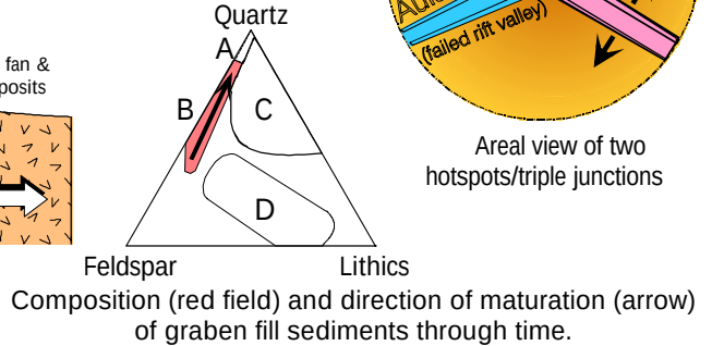
Foundering of Rift Valley / Marine Invasion
