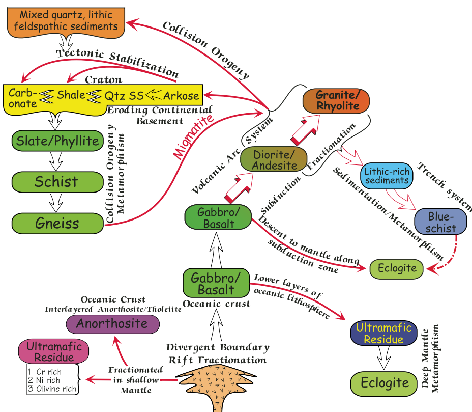
Figure 7. Tectonic Rock Cycle (after Fichter, 1996, 1999b), which illustrates the interconnected pathways between rock types related to their genesis in a particular tectonic setting. A divergent boundary (Fig. 5, stages B–D) produces basalt and gabbro, leaving behind ultramafic residue in the mantle. Initiation of a volcanic arc system produces diorite/andesite in island arc settings (Fig. 5, stage E) and granite/rhyolite in continental arc settings (Fig. 5, stage G). Subduction and metamorphism of oceanic crust and lithic-rich sediments produce blueschists and eclogites (Fig. 5, stages E and G). Mountain building along continental margins thickens the crust and produces Barrovian-style metamorphism of felsic sedimentary rocks, yielding slates, schists, and gneisses (Fig. 5, stages G–H). Tectonic stabilization enables extensive erosion of mountains that produces arkose, quartz sandstone, and shales and carbonates in shallow seas (Fig. 5, stage I).
