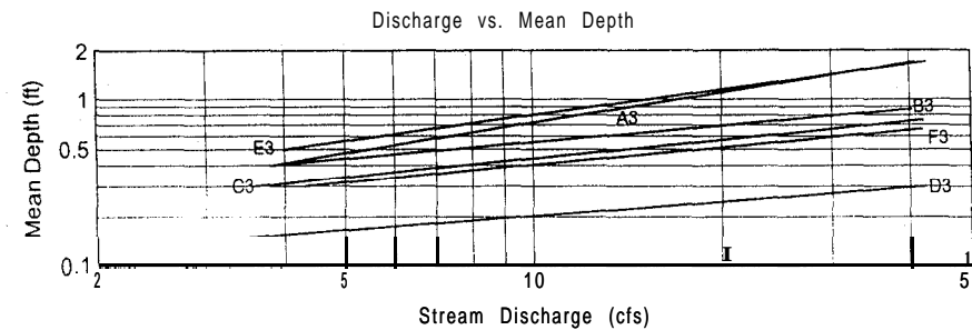
Fig. 11. Hydraulic geometry relations for selected stream types of uniform size.
